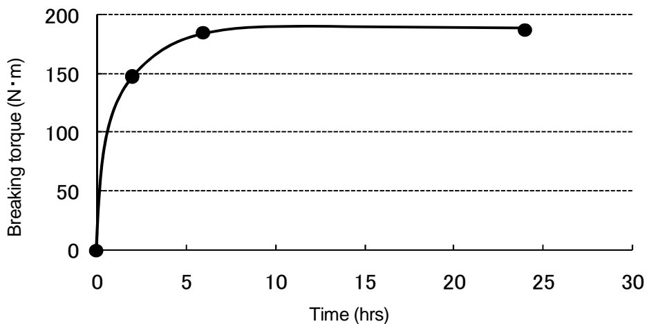
Fig. 3 Curing speed at room temperature Test piece: 3/4-in galvanized steel pipe Curing temperature: 25°C
