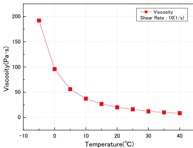
Fig. 2 Temperature-viscosity curve of TB1110F (shear rate: 10 (1/s))
