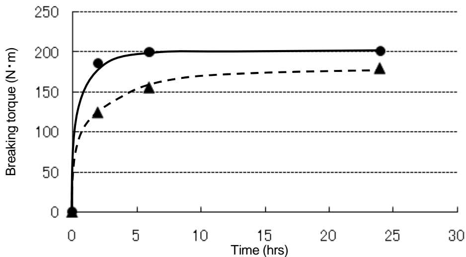
Fig. 4 Curing speed at low temperature Test piece: 3/4-in galvanized steel pipe Curing temperature: 5°C ● With use of primer (TB1390K) ▲ Without use of primer (TB1390K)
